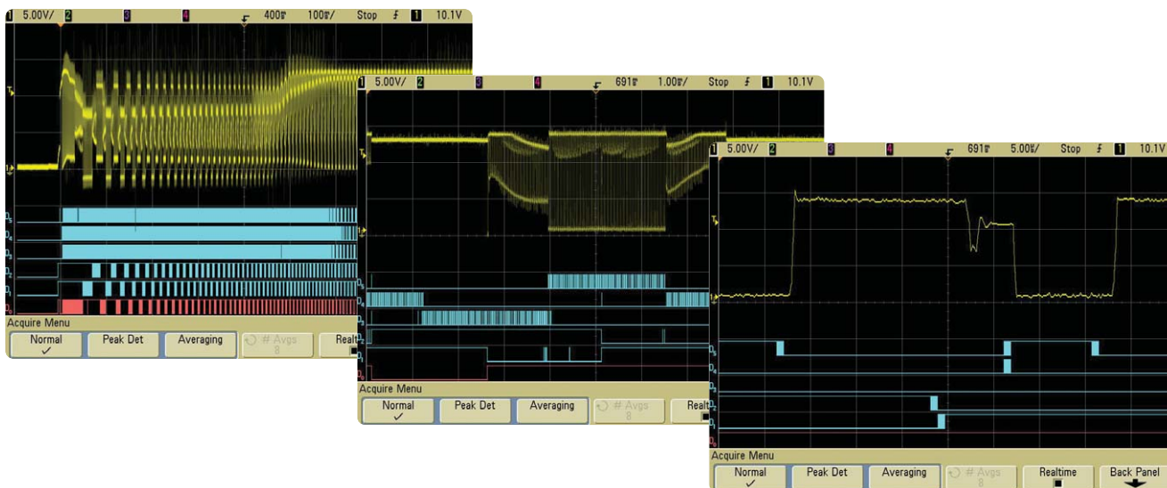
Figure 3. Motor drive signal start-up sequence with digital control signal triggering and various levels of zoom reveal "runt" pulse using Agilent's MS06000A Series MSOs.
